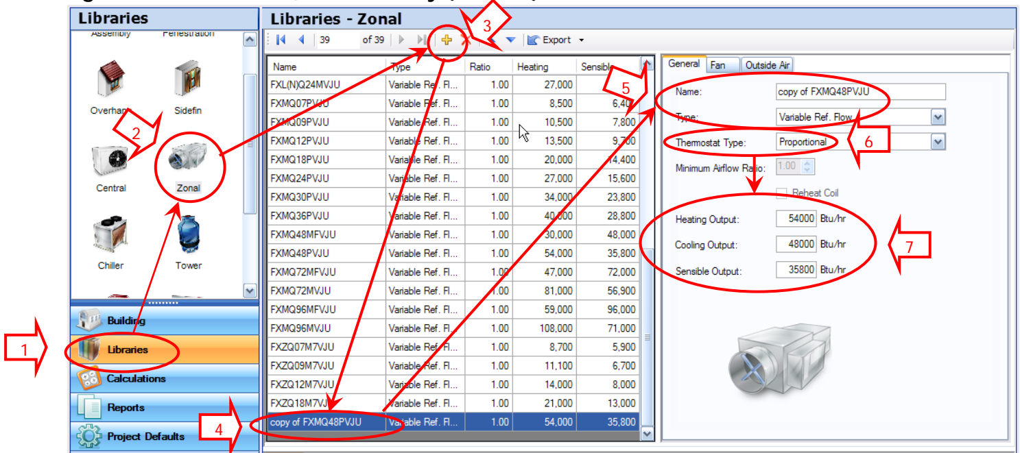
Figure 4: Indoor Units, Zonal Library (General)
