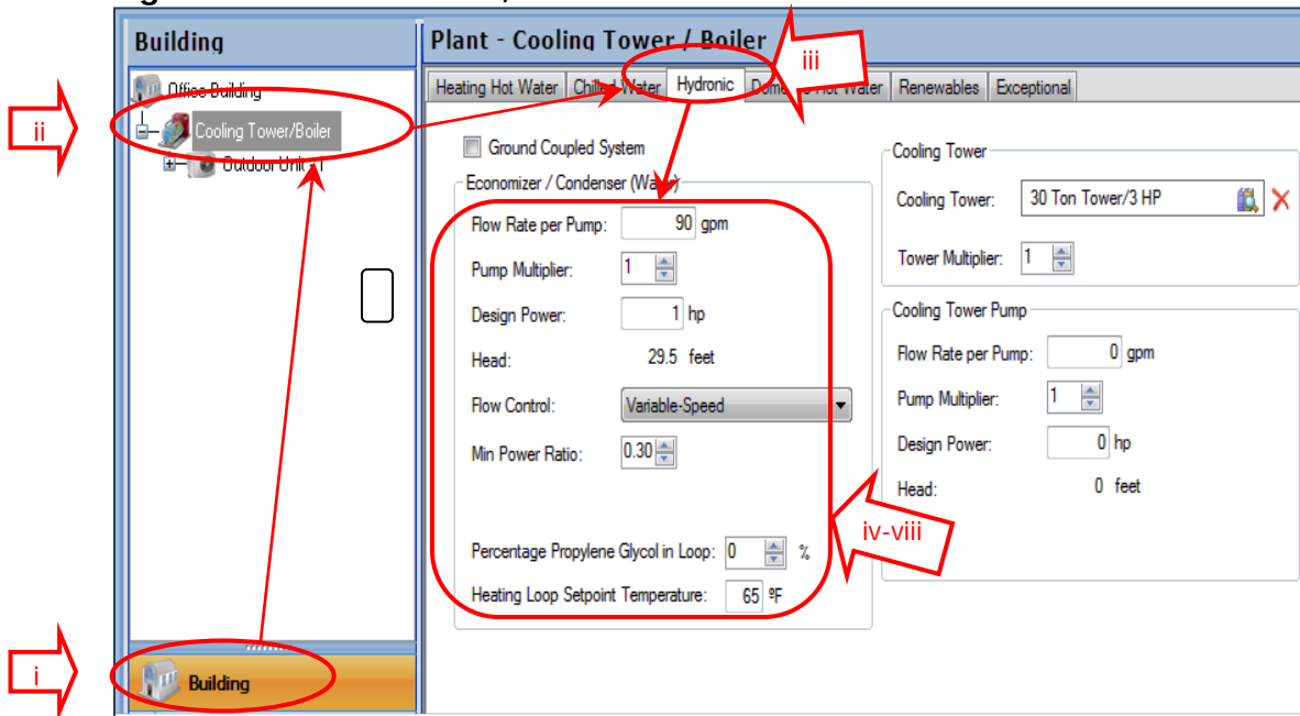
Figure 3: Plant Element, Water-Cooled Condenser
