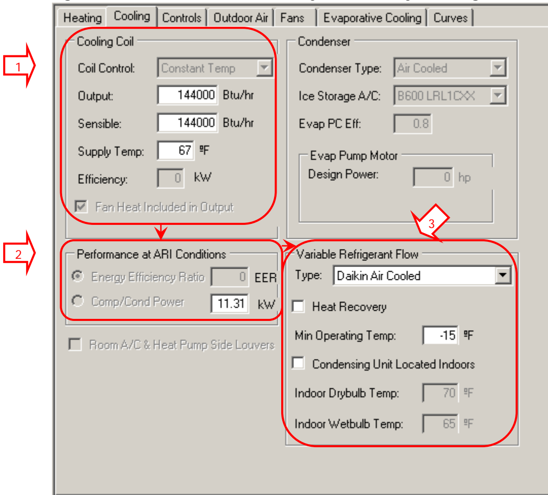
Figure 2: Outdoor Units, Central System Library, Cooling Tab
