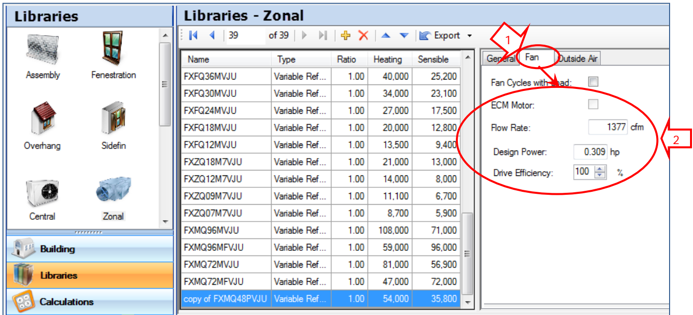
Figure 5: Indoor Units, Zonal Library (Fan)
